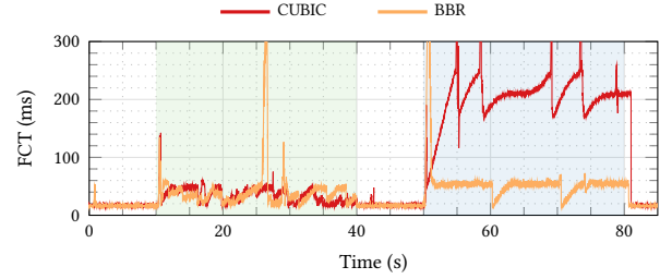
Figure 12: FCT comparison between a domestic client and AKS CH, showing the effects of parallel transfers and buffering with two CC algorithms. The delay-sensitive stream is characterized by 1 kB requests/responses exchanged every 10 ms; the green (10 s – 40 s) and blue (50 s – 80 s) shaded areas represent respectively parallel download and upload flows.
